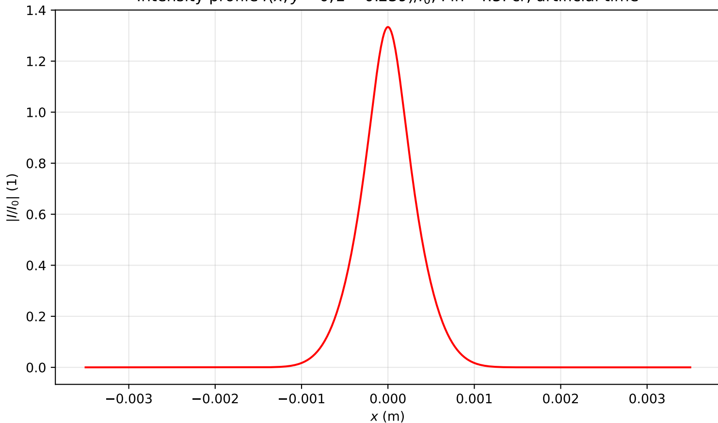
Intensity profile I(x, y = 0, z = 0.239)/I_0 , P_{in}=4.5P_{cr} , artificial time
